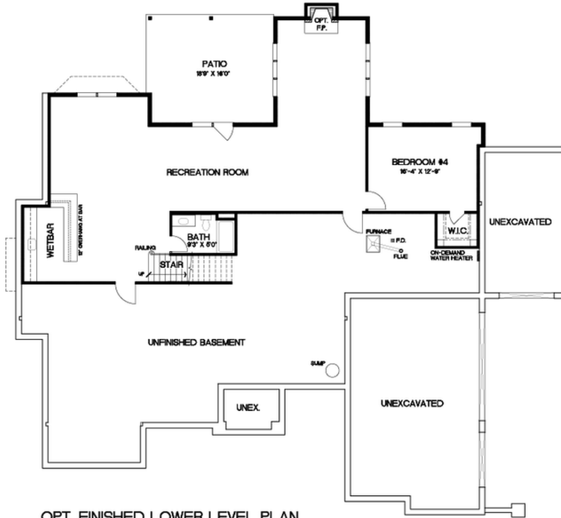
OPT. FINISHED LOWER LEVEL PLAN 1504 SF
